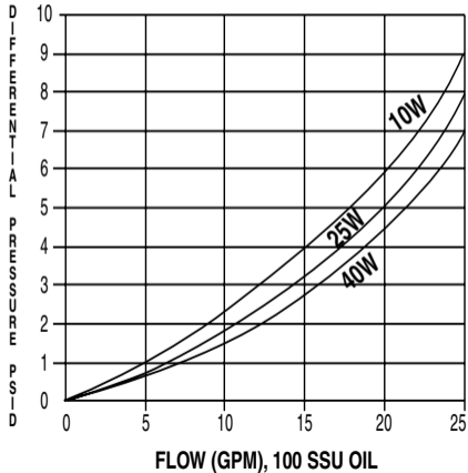
284 Series Stainless Elements
